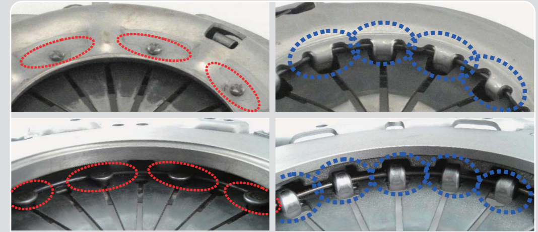
NVR Technology enables stronger spring support, resulting in better clutch control.
